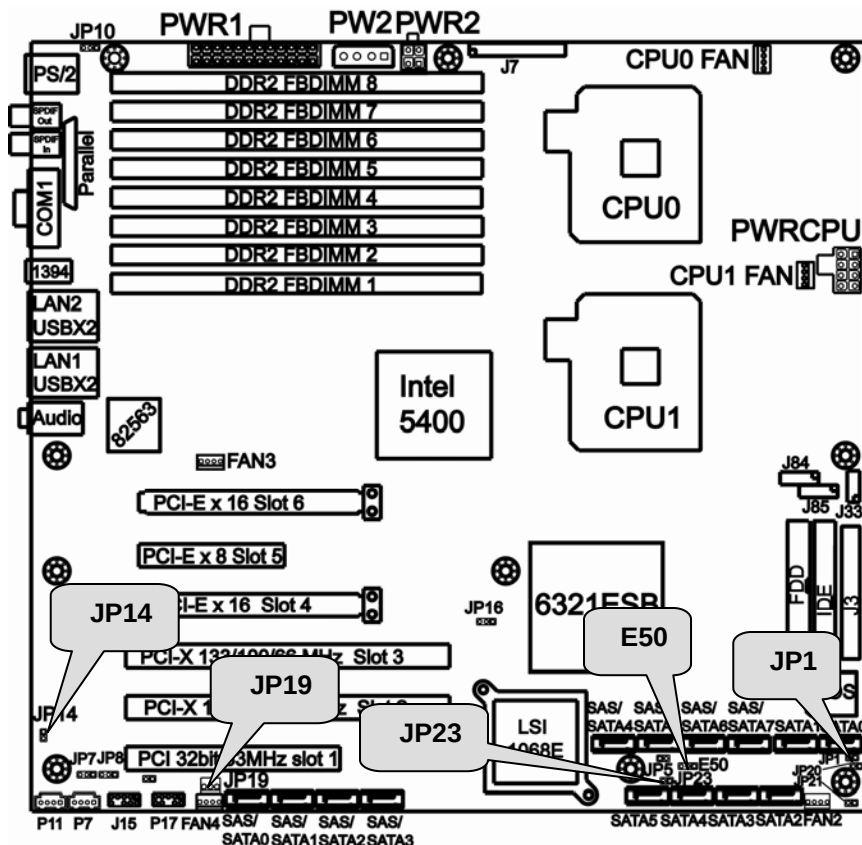
E50: CMOS Clear Jumper
