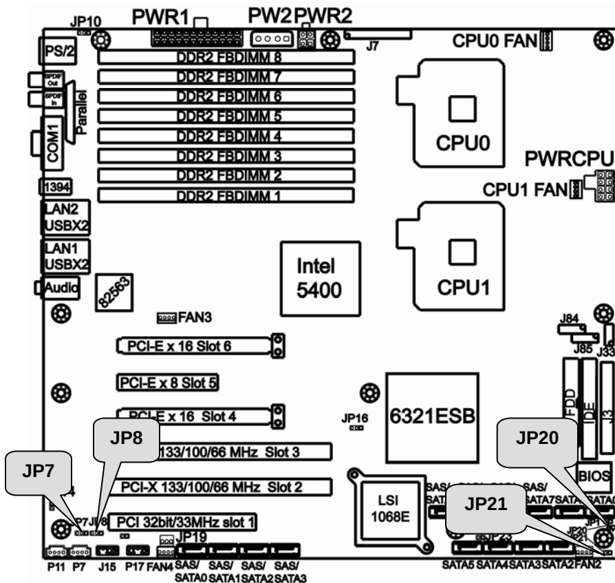
JP7/JP8: LAN Enable/Disable Jumper
