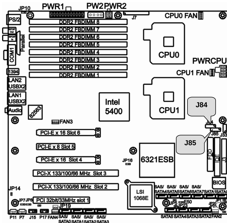
J84/J85: Front Panel USB 2.0 Connectors
