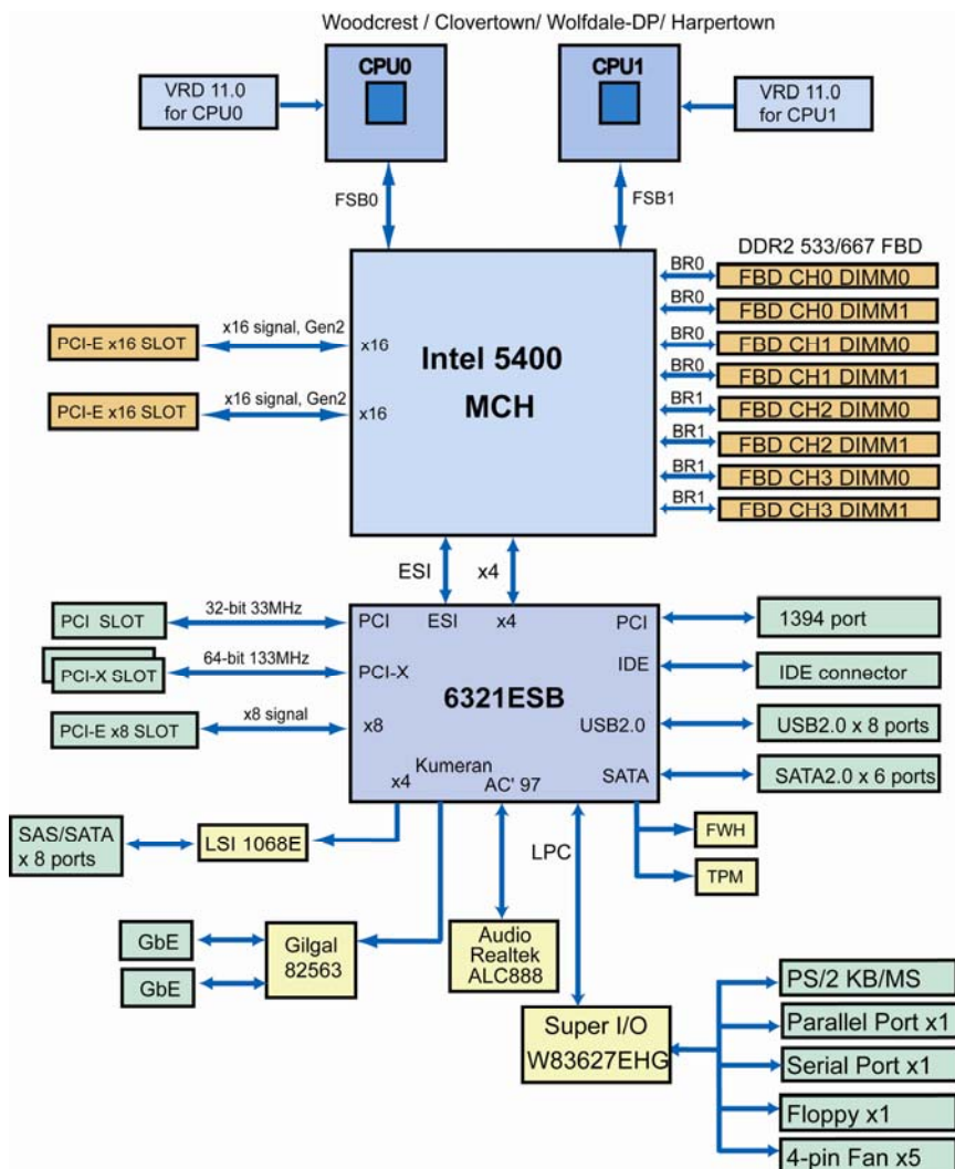
S5396 Block Diagram
