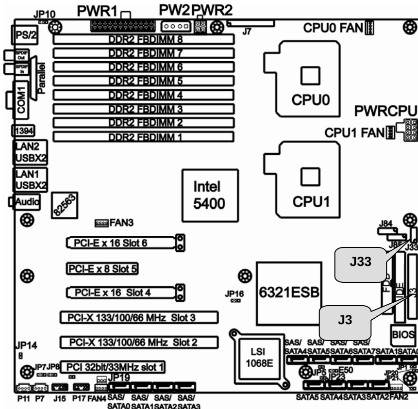
J33: 1394 Front Panel Header
