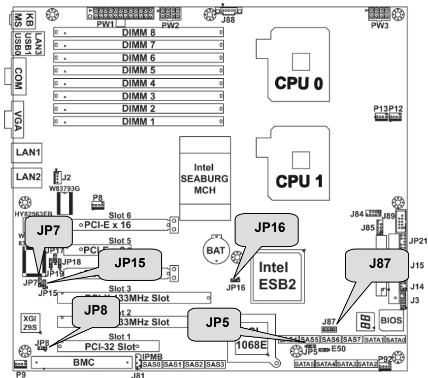
J87: Buzzer / External Speaker Header
